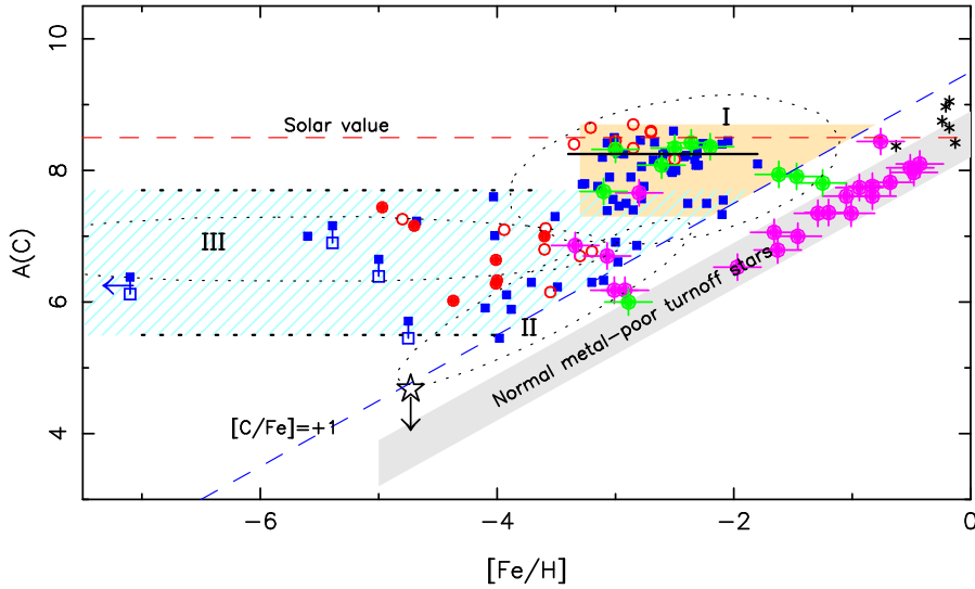
Fig. 8. Carbon abundance vs. [\text{Fe}/\text{H}] of the sample stars (pink and green dots show stars normal and rich in Ba, respectively). Red solid dots are the stars we analysed in the TOPoS project (Bonifacio et al. 2018); the open red dots are taken from Sivarani et al. (2006); Bonifacio et al. (2009, 2015); Spite et al. (2013); Behara et al. (2010); Sivarani et al. (2004) and Caffau et al. (2013a, 2016); the black star is taken from Caffau et al. (2012). The black asterisks show known CH dwarf stars (Karinkuzhi & Goswami 2014, 2015). The blue squares show stars from the literature (Yong et al. 2013; Cohen et al. 2003, 2013; Carollo et al. 2014; Masseron et al. 2012; Jonsell et al. 2006; Thompson et al. 2008; Hansen et al. 2015, 2016; Lucatello et al. 2003; Aoki et al. 2002, 2006, 2008; Frebel et al. 2005; Li et al. 2015; Norris et al. 2007; Christlieb et al. 2004; Keller et al. 2014; Frebel et al. 2015; Roederer et al. 2014; Ivans et al. 2005). The blue and orange areas in the figure highlight the two carbon bands as defined in Bonifacio et al. (2018). The black dashed ellipses represent the regions containing the three CEMP populations according to Yoon et al. (2016).
