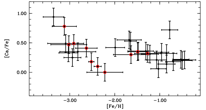
Fig. 6. [Ca/Fe] derived from the Ca II-K line vs. [Fe/H] . The black dots surrounded by a red corona represent Ba-rich stars. The solar A(Fe) value of 7.52 is taken from Caffau et al. (2011) , and the solar A(Ca) = 6.33 is adopted from Lodders et al. (2009) .
