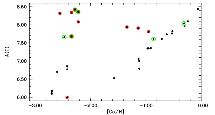
Fig. 7. Carbon abundance vs. [Ca/H] derived from the Ca II-K line. The black dots surrounded by a red corona represent Ba-rich stars. An extra green corona is used in the cases of uncertain measurements. Downward arrows represent upper limits.
