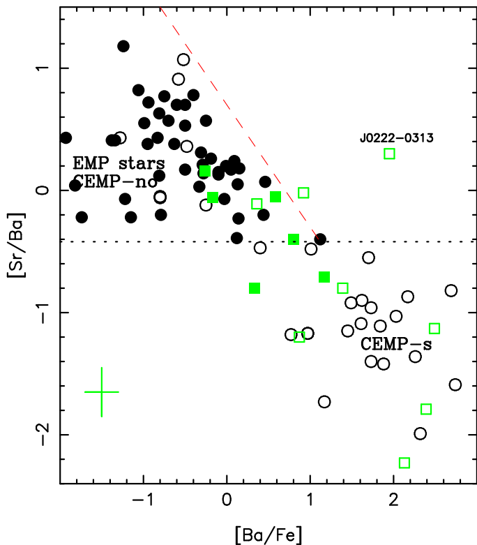
Fig. 9. [\text{Sr}/\text{Ba}] ratio vs. [\text{Ba}/\text{Fe}] . The black filled circles represent the normal EMP dwarfs and giants studied in the frame of the ESO Large Programme First Stars (Cayrel et al. 2004; Bonifacio et al. 2009) and the stars studied homogeneously by Siqueira-Mello et al. (2015). The black open circles are for CEMP stars studied in the frame of this ESO Large Programme or taken from the literature (Depagne et al. 2002; Sivarani et al. 2004, 2006; Barbuy et al. 2005; Behara et al. 2010; Spite et al. 2013; Yong et al. 2013). The green filled squares show normal metal-poor stars studied in this paper, and the open green squares denote the C-rich stars. Note the very peculiar position of the CEMP star SDSS J0222-0313. In this star the first-peak heavy elements (such as Sr) seem to be more enriched than the second-peak heavy elements (like Ba).
