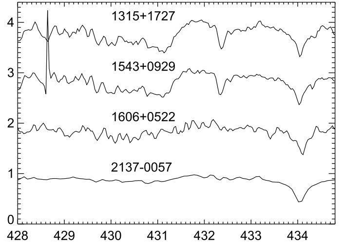
Fig. 1. Observed spectra for four stars in the range of the G -band.
