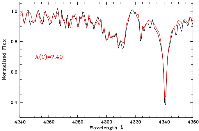
Fig. 4. Observed spectrum of SDSS J0905+0330 (solid black) compared with the best fit (solid red) based on a 3D synthesis of a model that is 21 K cooler.
