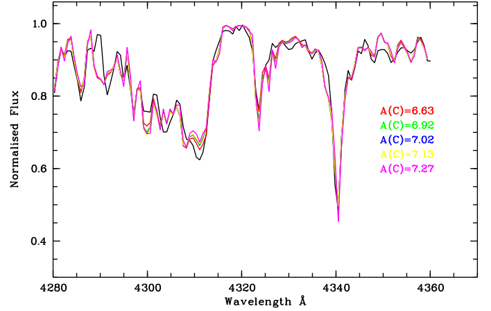
Fig. 5. Observed spectrum of SDSS J1313–0010 (solid black) compared with the best fit based on a 3D synthesis with various C/O content. The pink profile corresponds to A(C) - A(O) = -1.67 , and the red profile shows A(C) - A(O) = +0.33 .
