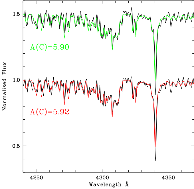
Fig. 3. Two observed spectra of SDSS J1445–0045 (solid black) compared with the best fit (solid green and red) based on a 3D synthesis of a model that is 18 K cooler.
