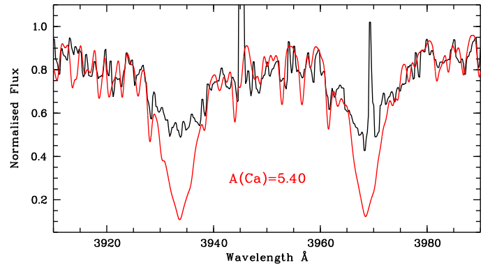
Fig. 2. Observed spectrum of SDSS J1114–1202 (solid black) compared with a synthetic spectrum (solid red) with A(\text{Ca}) compatible with the value derived from the other two Ca I lines and with A(\text{Fe}) .
