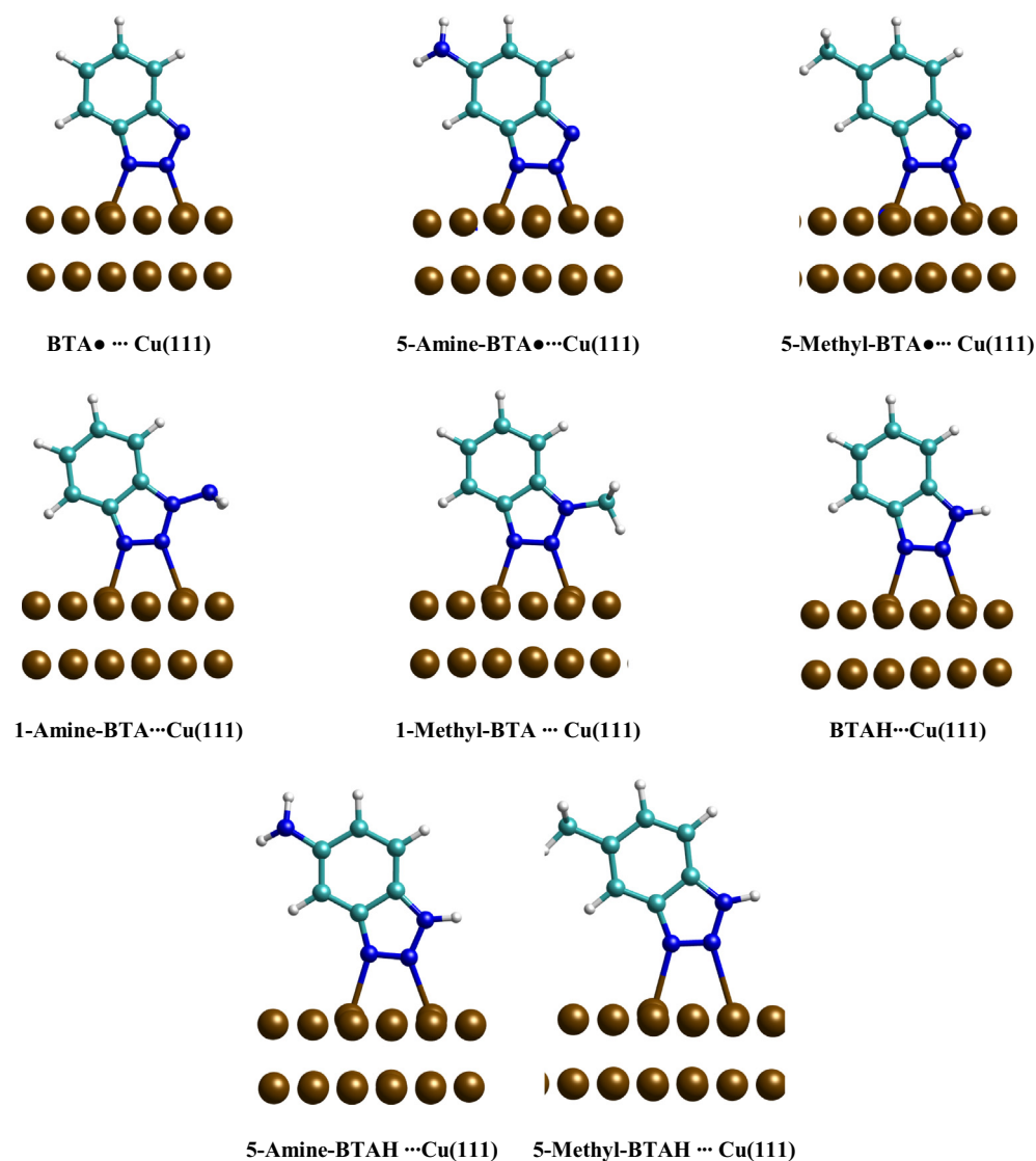
Fig. 2. The most stable BTA(H) -Cu(111) complexes obtained using the PBE method. In the ball-and-stick representation, carbon, nitrogen, hydrogen and copper atoms are colored in green, blue, white and brown respectively. (For interpretation of the references to colour in this figure legend, the reader is referred to the web version of this article.)
