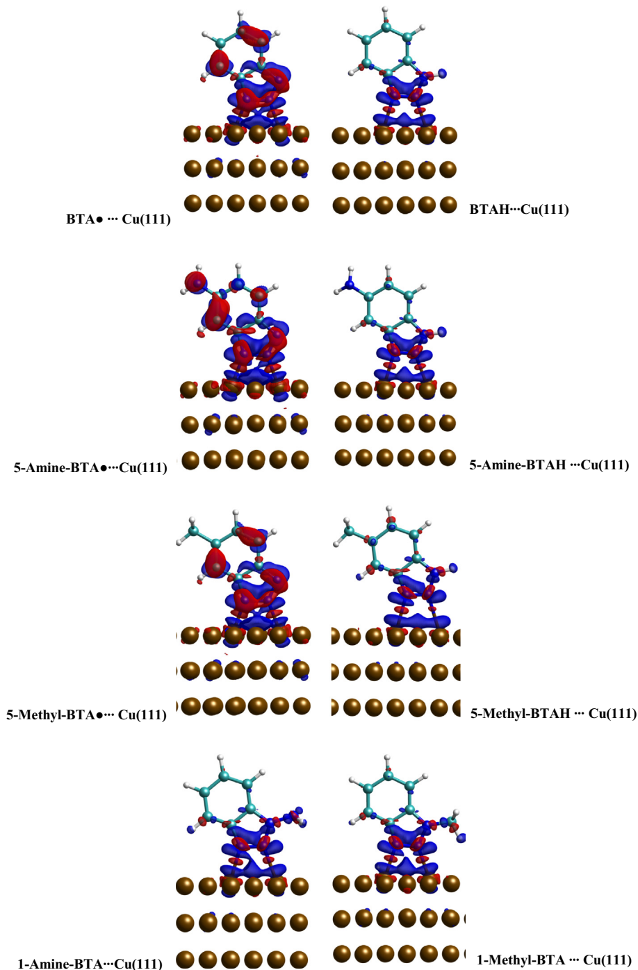
Fig. 3. Charge density difference for the most stable BTA(H) -Cu(1 1 1) complexes. The blue (red) color represents the electron deficit (excess) regions, i.e., charge flows from blue to red regions. (For interpretation of the references to colour in this figure legend, the reader is referred to the web version of this article.)
