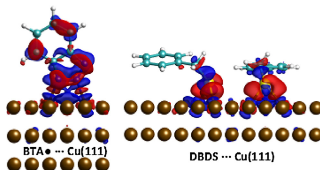
Fig. 4. Charge density difference for BTA● and DBDS adsorbed on Cu(111) surface.
