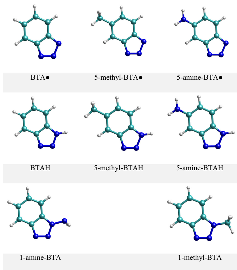
Fig. 1. Structures of radical and molecular benzotriazole derivatives. In the ball-and-stick representation, carbon, nitrogen, and hydrogen atoms are colored in green, blue, and white, respectively. (For interpretation of the references to colour in this figure legend, the reader is referred to the web version of this article.)
